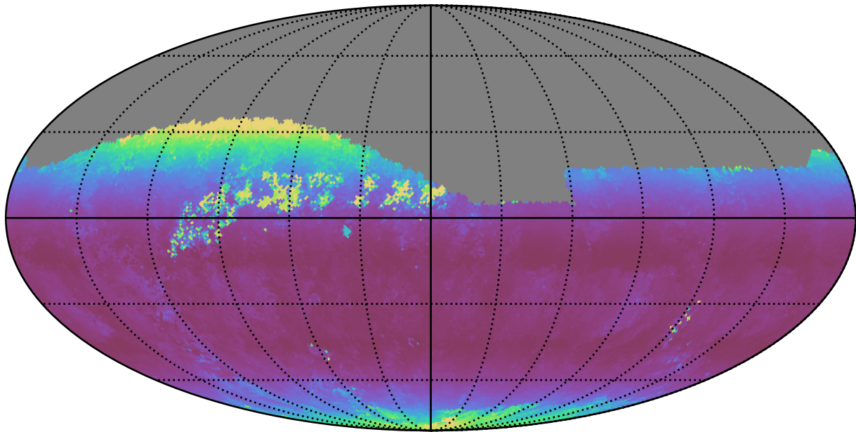
weather_cloudso35v3.4_10yrs Yr 1 r band: Median airmass
