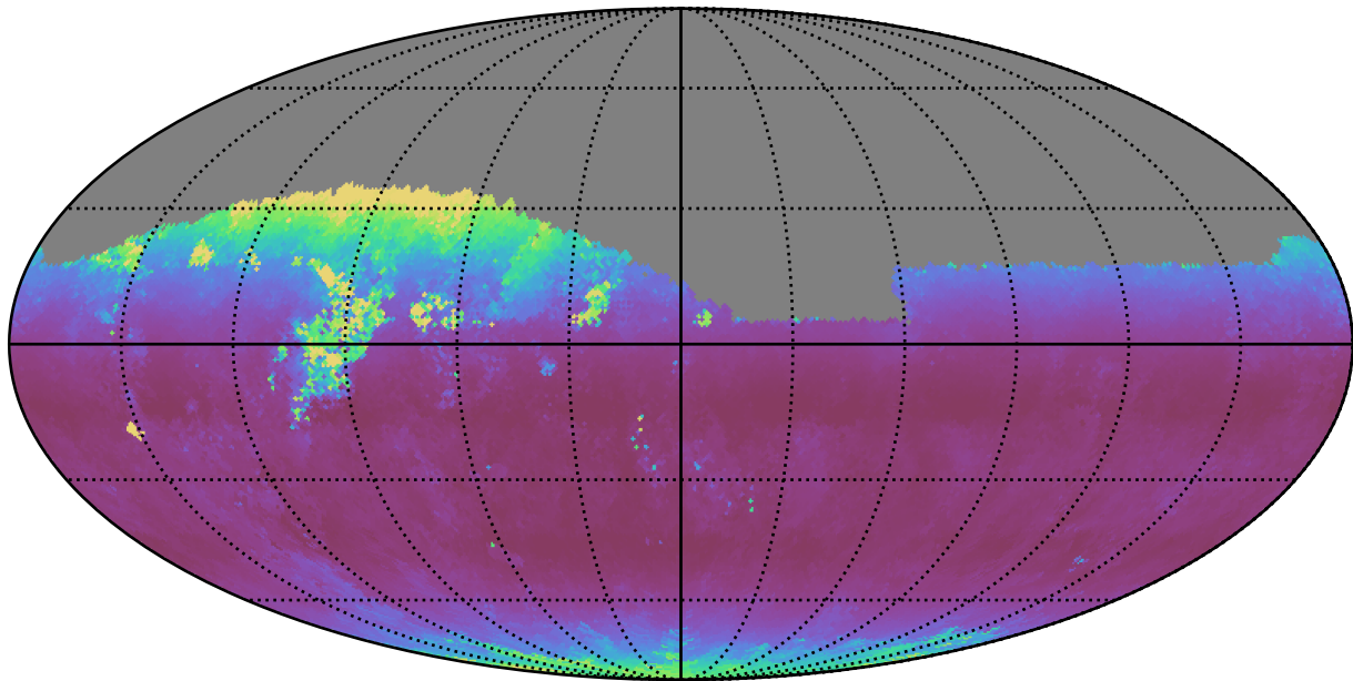
weather_cloudso35v3.4_10yrs Yr 1 i band: Median airmass
