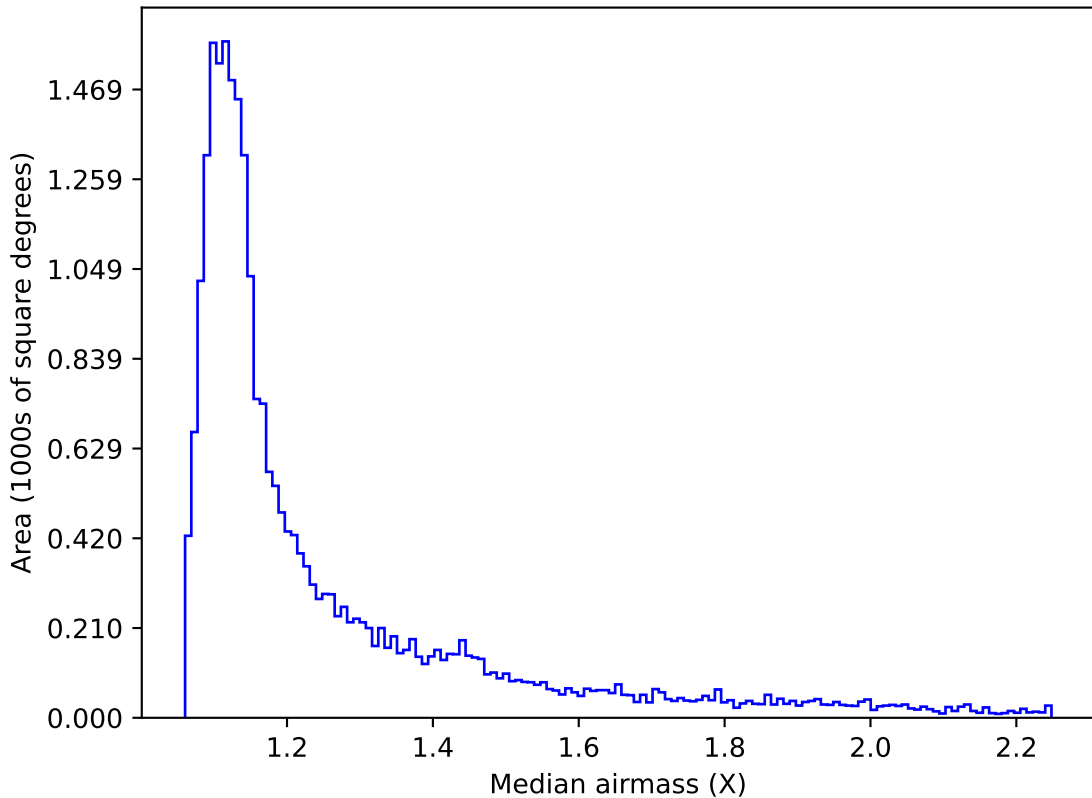
weather_cloudso35v3.4_10yrs Yr 1 i band: Median airmass
