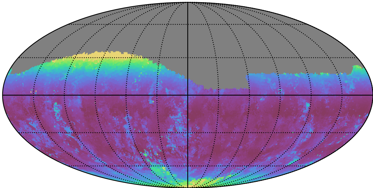
weather_cloudso35v3.4_10yrs Yr 1 g band: Median airmass
