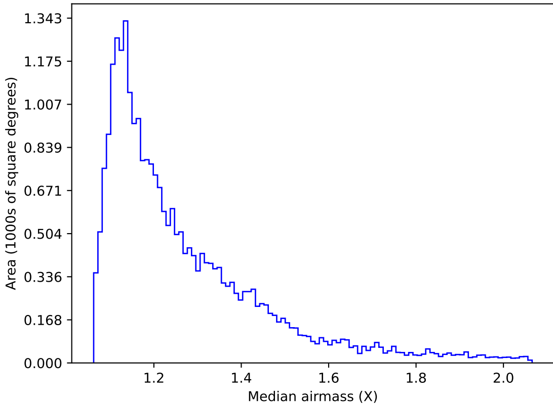
weather_cloudso35v3.4_10yrs Yr 1 g band: Median airmass
