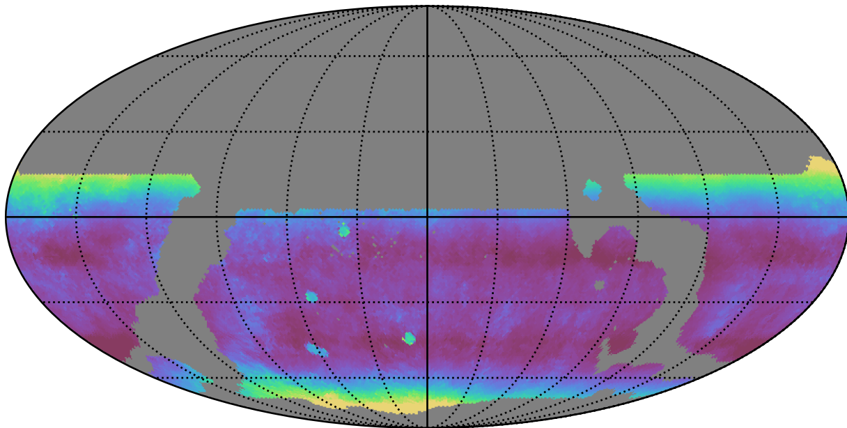
weather_cloudso35v3.4_10yrs WFD z band: Median airmass
