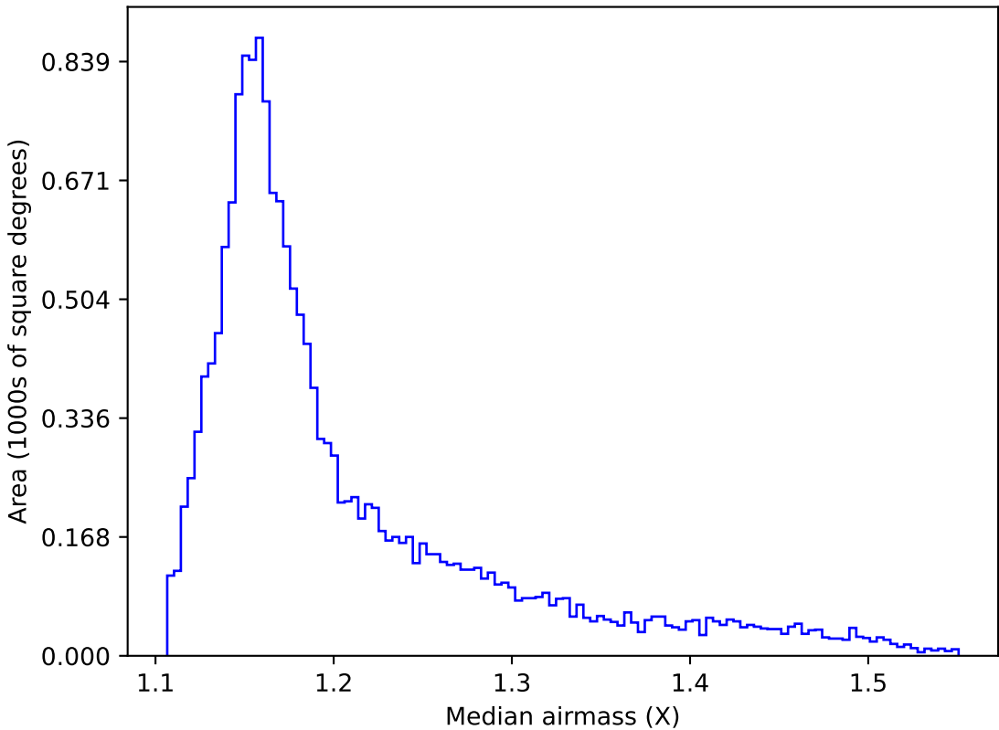
weather_cloudso35v3.4_10yrs WFD y band: Median airmass
