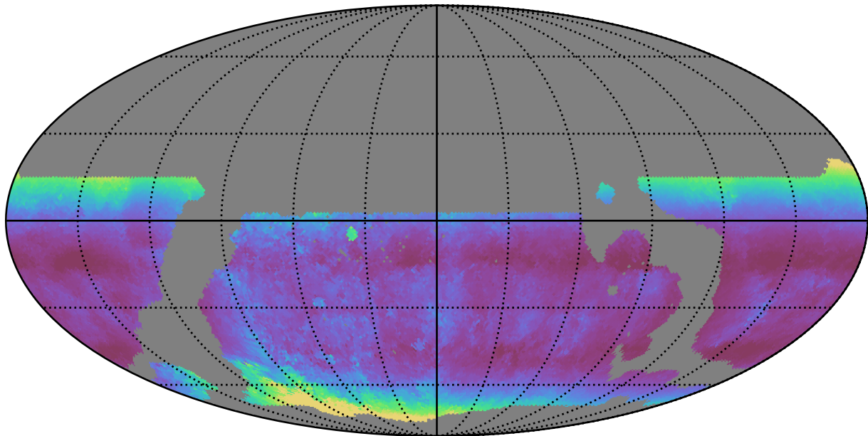
weather_cloudso35v3.4_10yrs WFD u band: Median airmass
