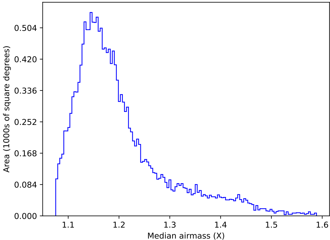
weather_cloudso35v3.4_10yrs WFD u band: Median airmass
