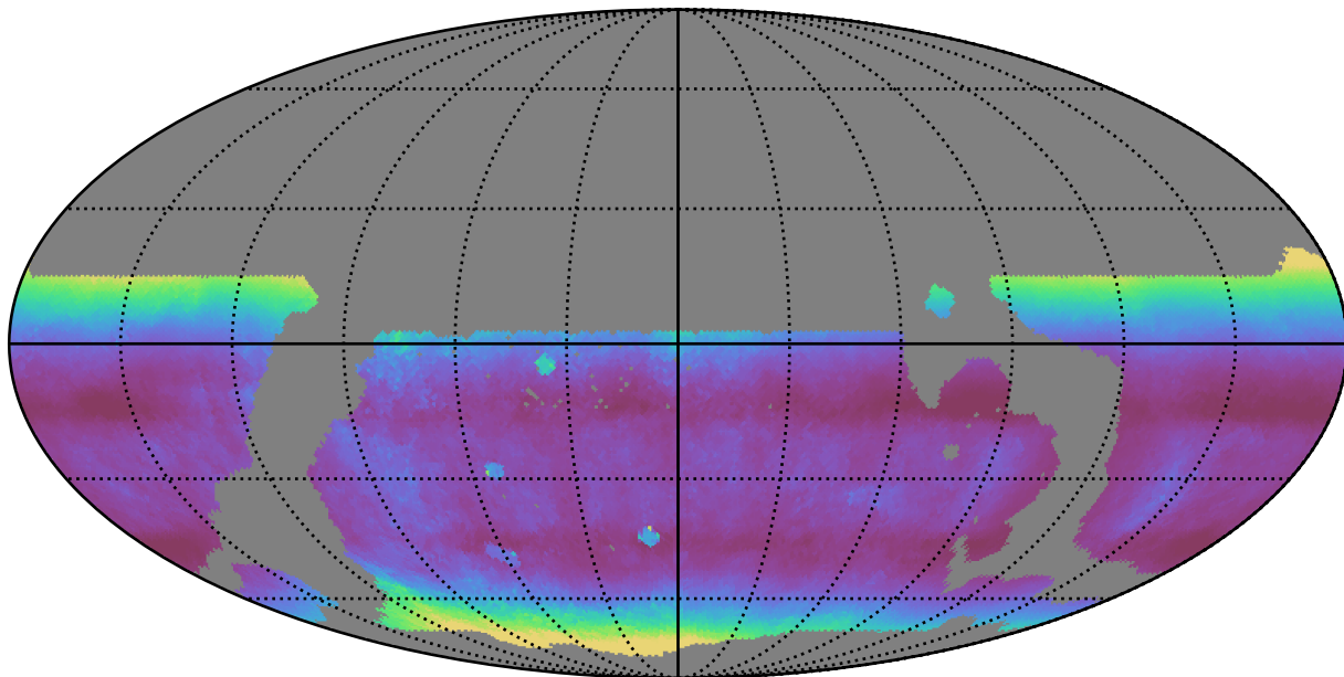
weather_cloudso35v3.4_10yrs WFD r band: Median airmass
