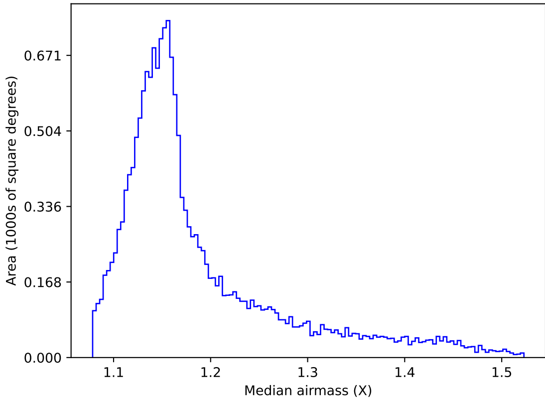
weather_cloudso35v3.4_10yrs WFD r band: Median airmass
