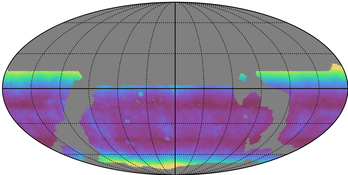
weather_cloudso35v3.4_10yrs WFD i band: Median airmass
