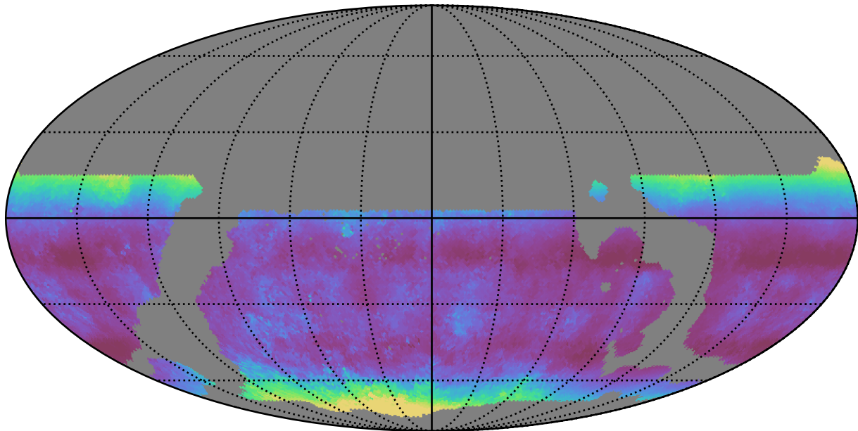
weather_cloudso35v3.4_10yrs WFD g band: Median airmass
