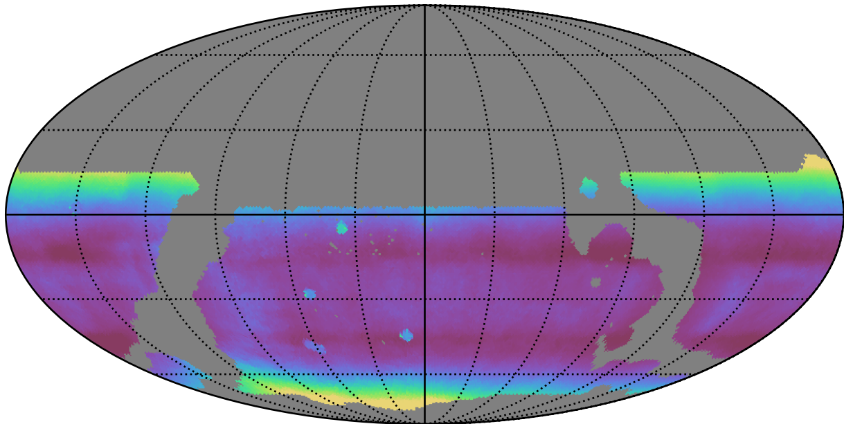
weather_cloudso35v3.4_10yrs WFD all bands: Median airmass
