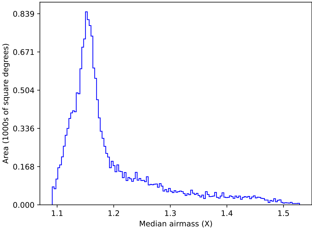
weather_cloudso35v3.4_10yrs WFD all bands: Median airmass
