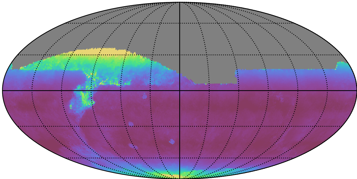
weather_cloudso35v3.4_10yrs All sky z band: Median airmass
