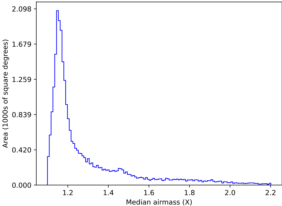
weather_cloudso35v3.4_10yrs All sky z band: Median airmass
