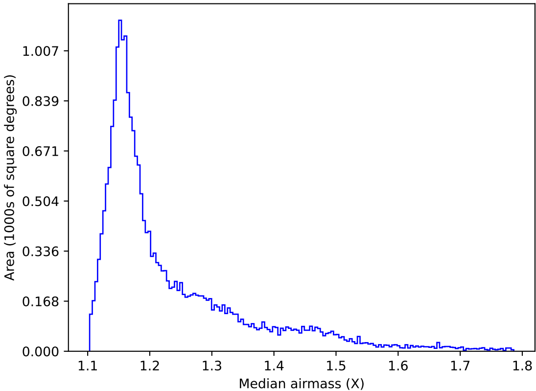
weather_cloudso35v3.4_10yrs All sky y band: Median airmass
