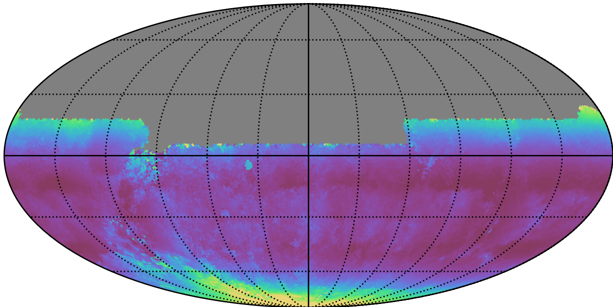
weather_cloudso35v3.4_10yrs All sky u band: Median airmass
