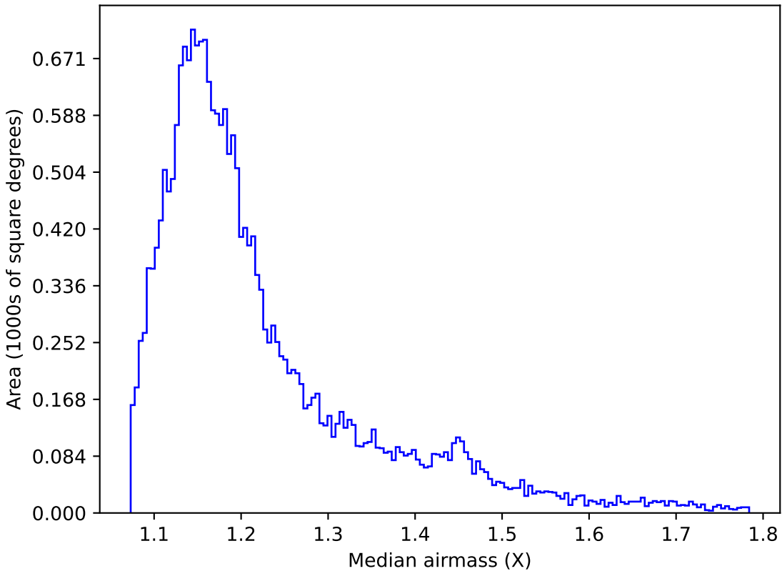
weather_cloudso35v3.4_10yrs All sky u band: Median airmass
