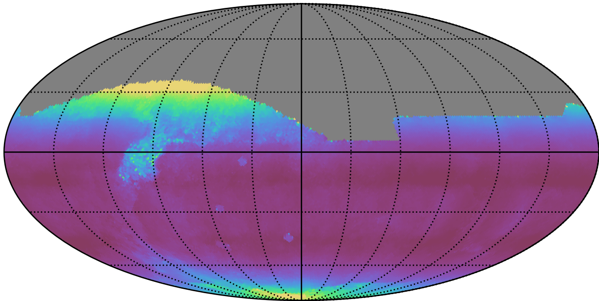
weather_cloudso35v3.4_10yrs All sky r band: Median airmass
