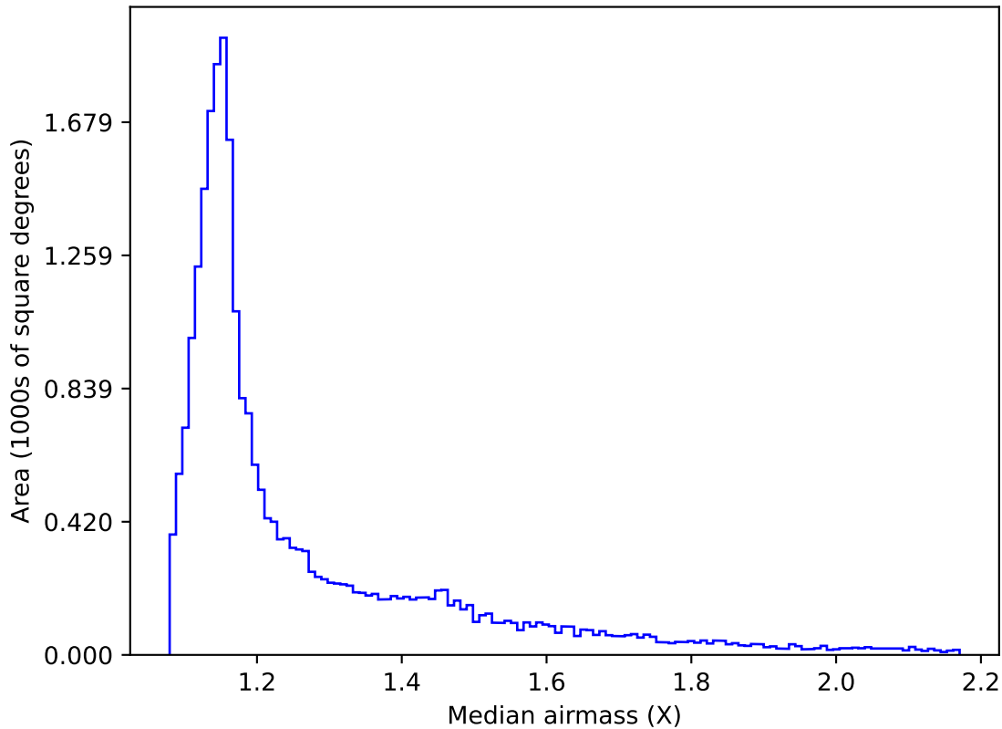
weather_cloudso35v3.4_10yrs All sky r band: Median airmass
