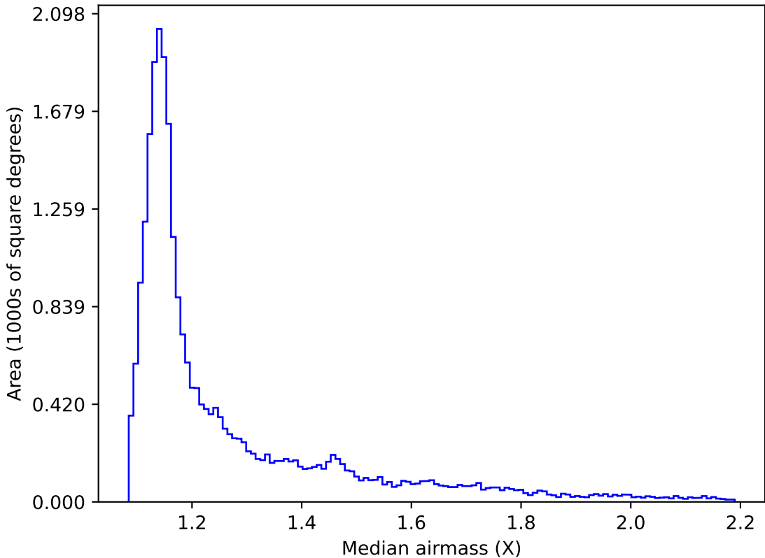
weather_cloudso35v3.4_10yrs All sky i band: Median airmass
