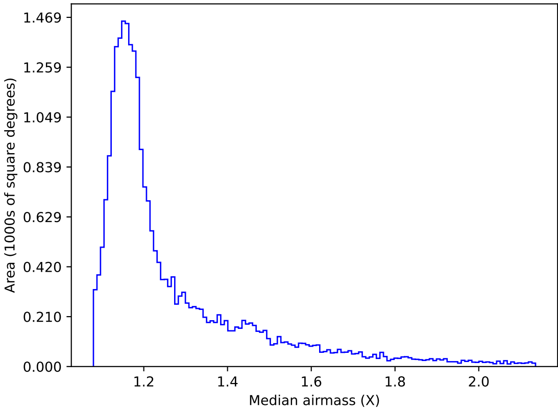
weather_cloudso35v3.4_10yrs All sky g band: Median airmass
