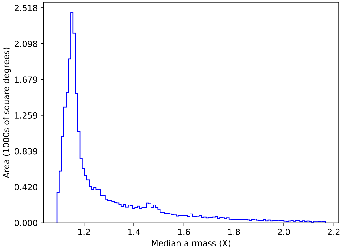
weather_cloudso35v3.4_10yrs All sky all bands: Median airmass
