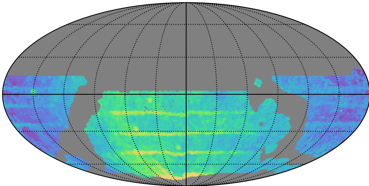
weather_cloudso35v3.4_10yrs WFD z band: Median Season Length
