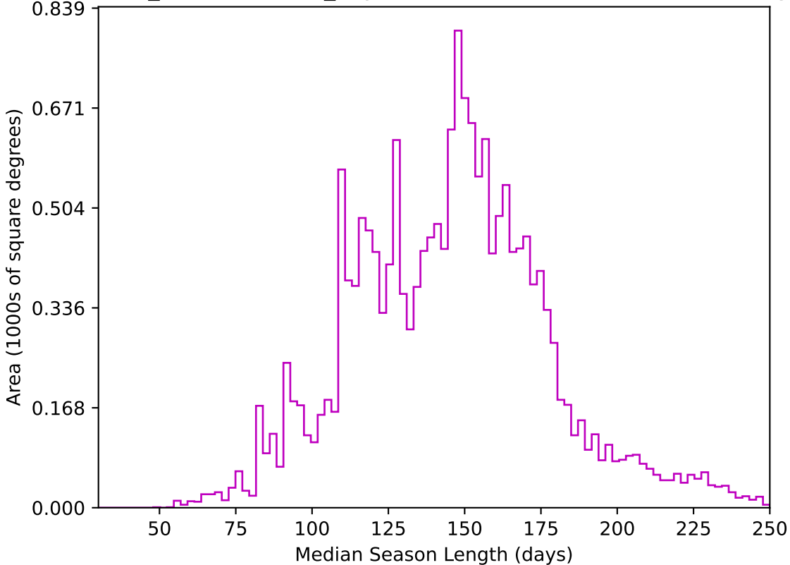
weather_cloudso35v3.4_10yrs WFD z band: Median Season Length
