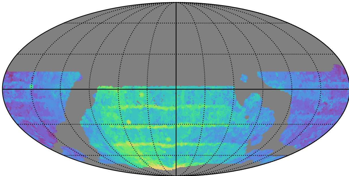
weather_cloudso35v3.4_10yrs WFD y band: Median Season Length
