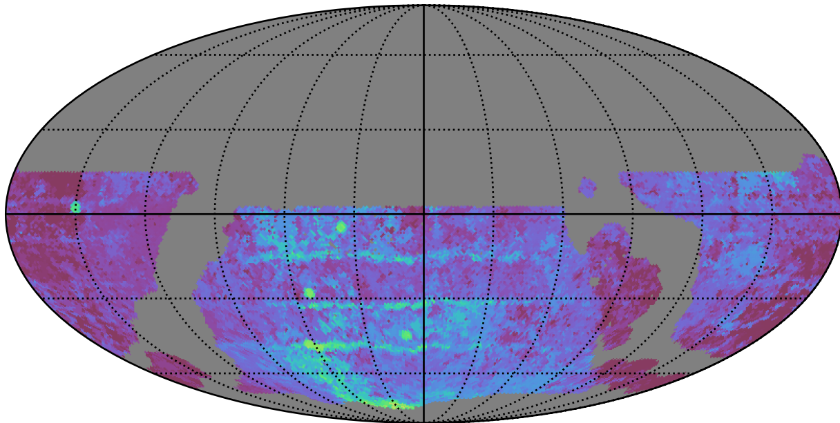
weather_cloudso35v3.4_10yrs WFD u band: Median Season Length
