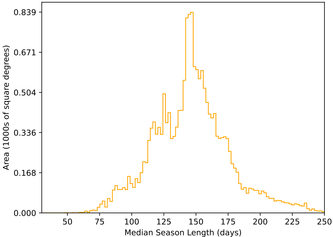
weather_cloudso35v3.4_10yrs WFD r band: Median Season Length
