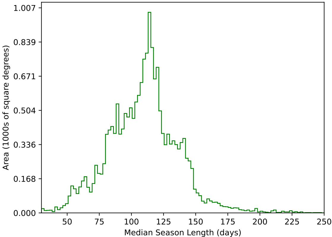
weather_cloudso35v3.4_10yrs WFD g band: Median Season Length
