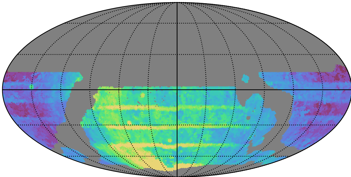
weather_cloudso35v3.4_10yrs WFD all bands: Median Season Length
