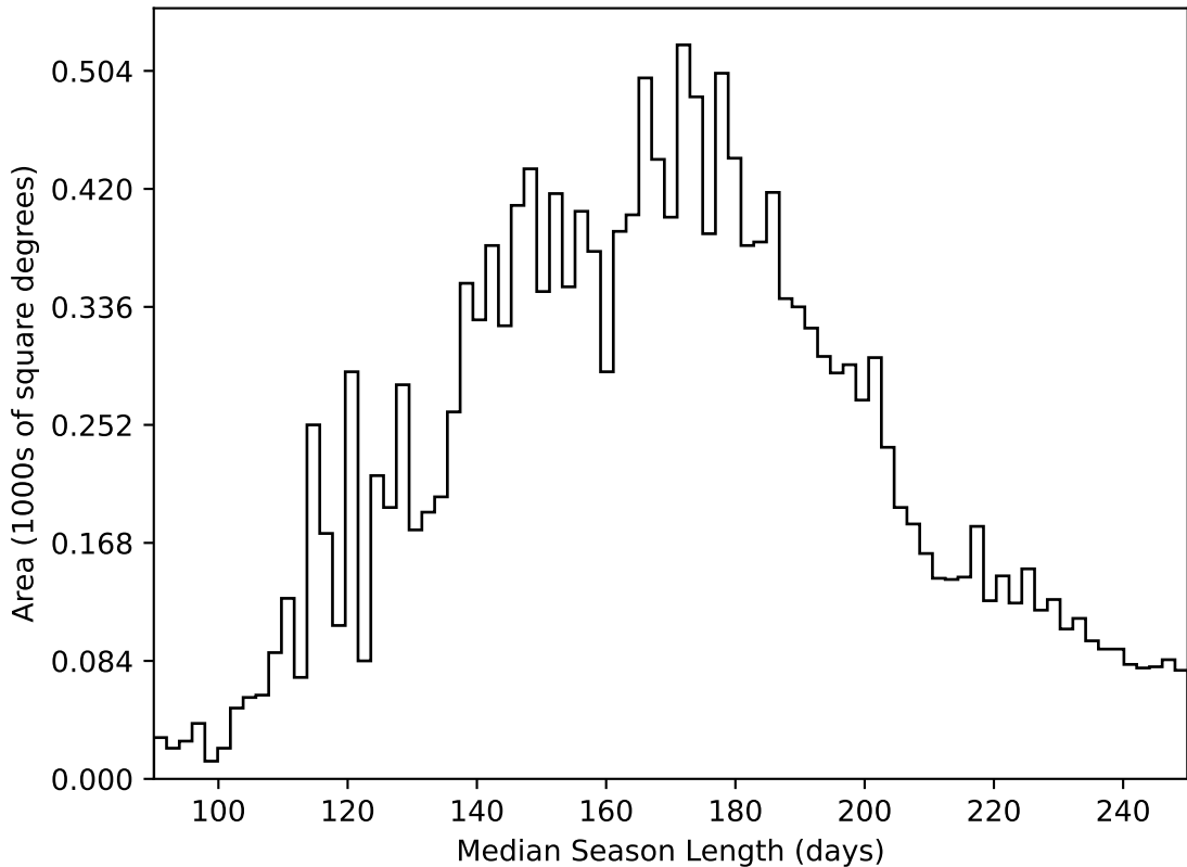
weather_cloudso35v3.4_10yrs WFD all bands: Median Season Length
