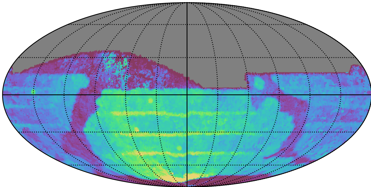
weather_cloudso35v3.4_10yrs All sky z band: Median Season Length
