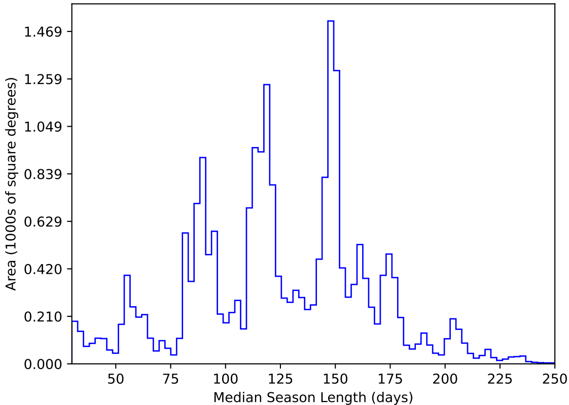
weather_cloudso35v3.4_10yrs All sky y band: Median Season Length
