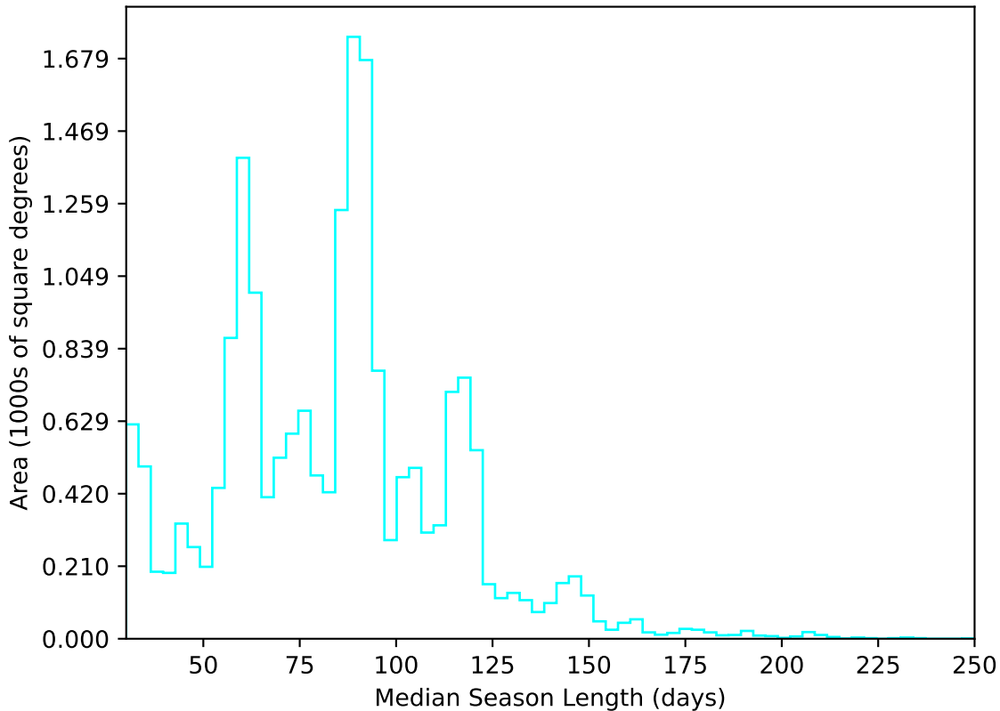
weather_cloudso35v3.4_10yrs All sky u band: Median Season Length
