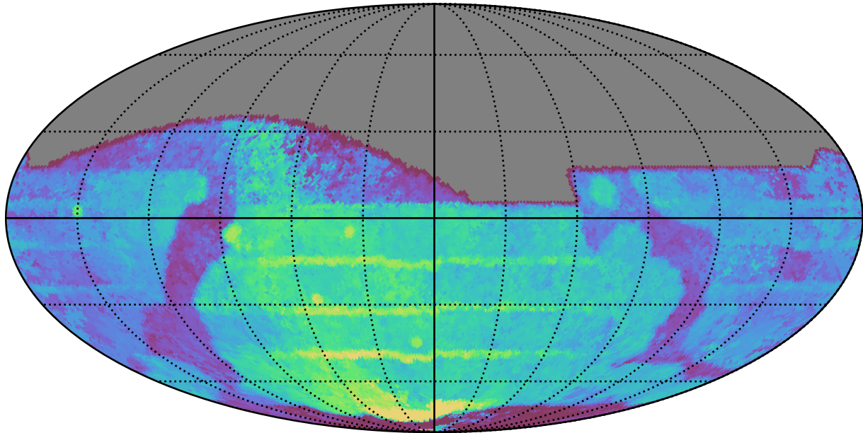
weather_cloudso35v3.4_10yrs All sky i band: Median Season Length
