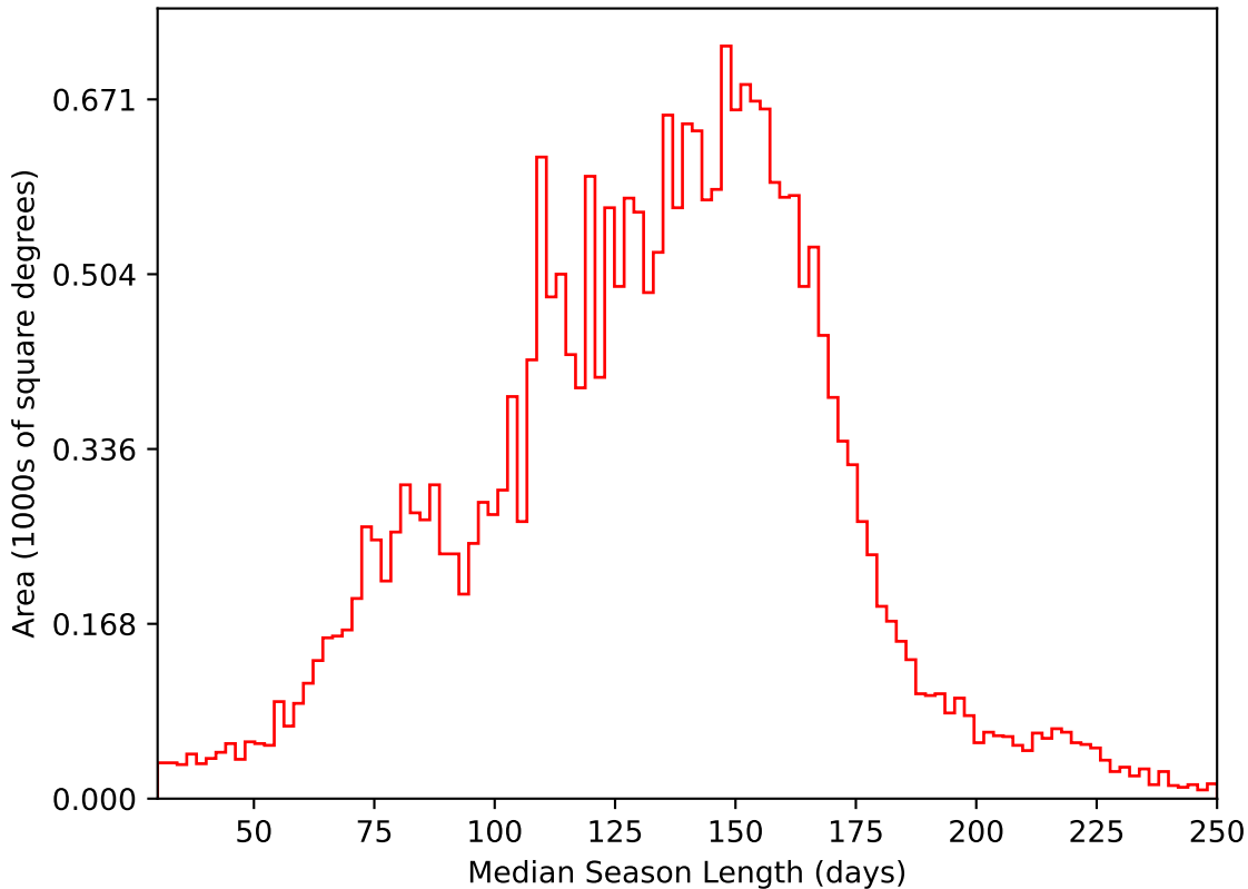
weather_cloudso35v3.4_10yrs All sky i band: Median Season Length
