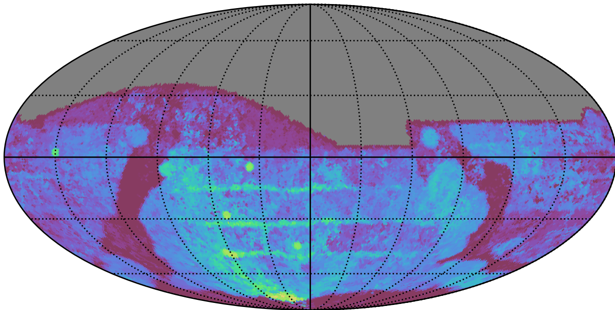
weather_cloudso35v3.4_10yrs All sky g band: Median Season Length
