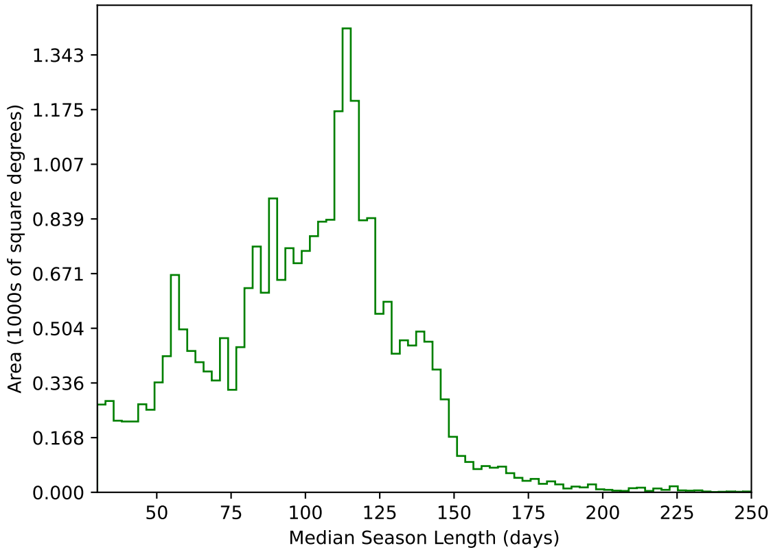
weather_cloudso35v3.4_10yrs All sky g band: Median Season Length
