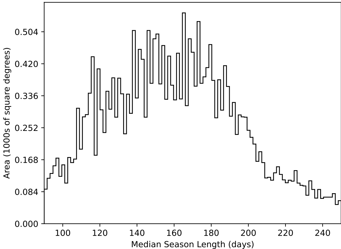
weather_cloudso35v3.4_10yrs All sky all bands: Median Season Length
