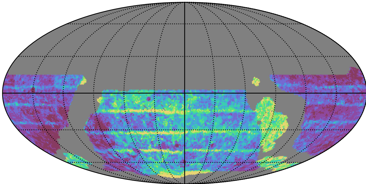
weather_cloudso35v3.4_10yrs WFD z band: Median Inter-Night Gap
