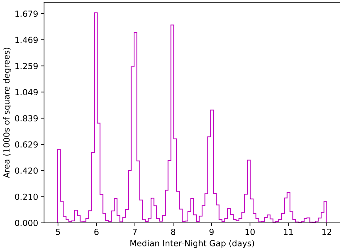
weather_cloudso35v3.4_10yrs WFD z band: Median Inter-Night Gap
