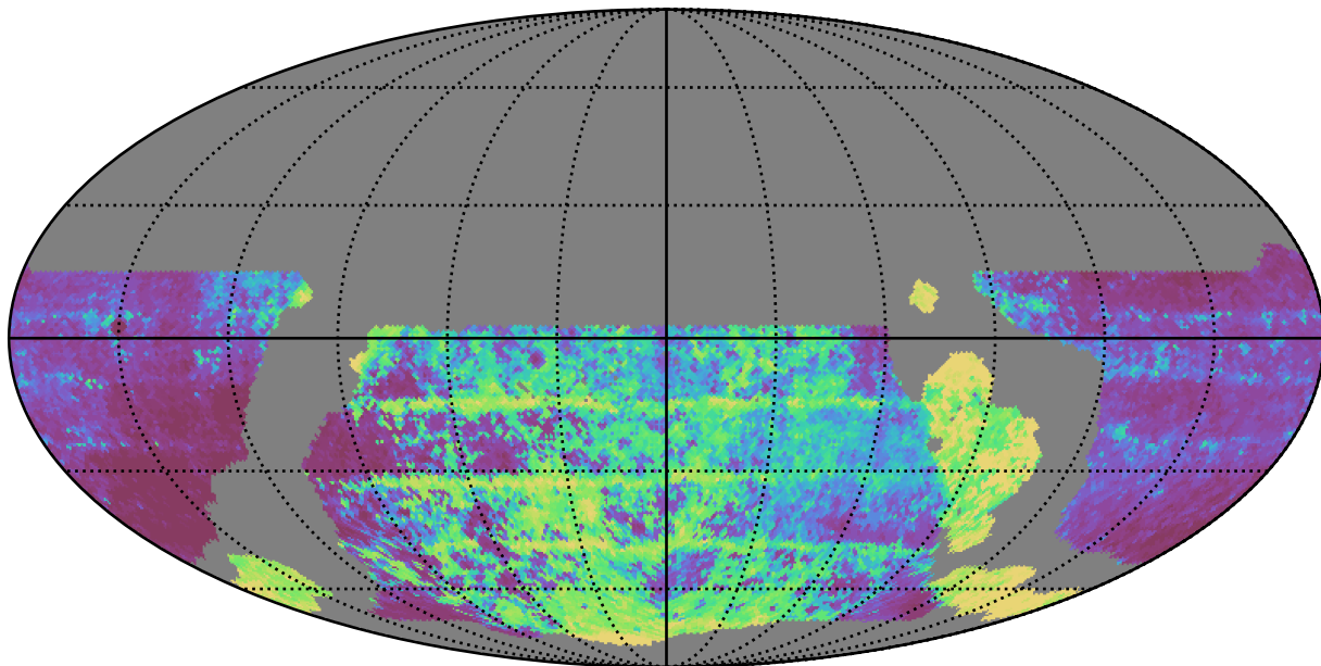
weather_cloudso35v3.4_10yrs WFD y band: Median Inter-Night Gap
