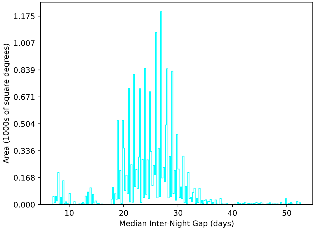
weather_cloudso35v3.4_10yrs WFD u band: Median Inter-Night Gap
