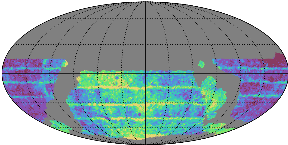
weather_cloudso35v3.4_10yrs WFD i band: Median Inter-Night Gap
