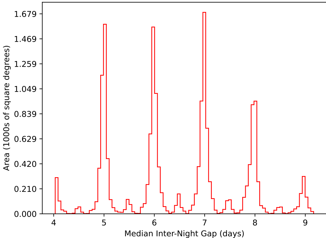
weather_cloudso35v3.4_10yrs WFD i band: Median Inter-Night Gap
