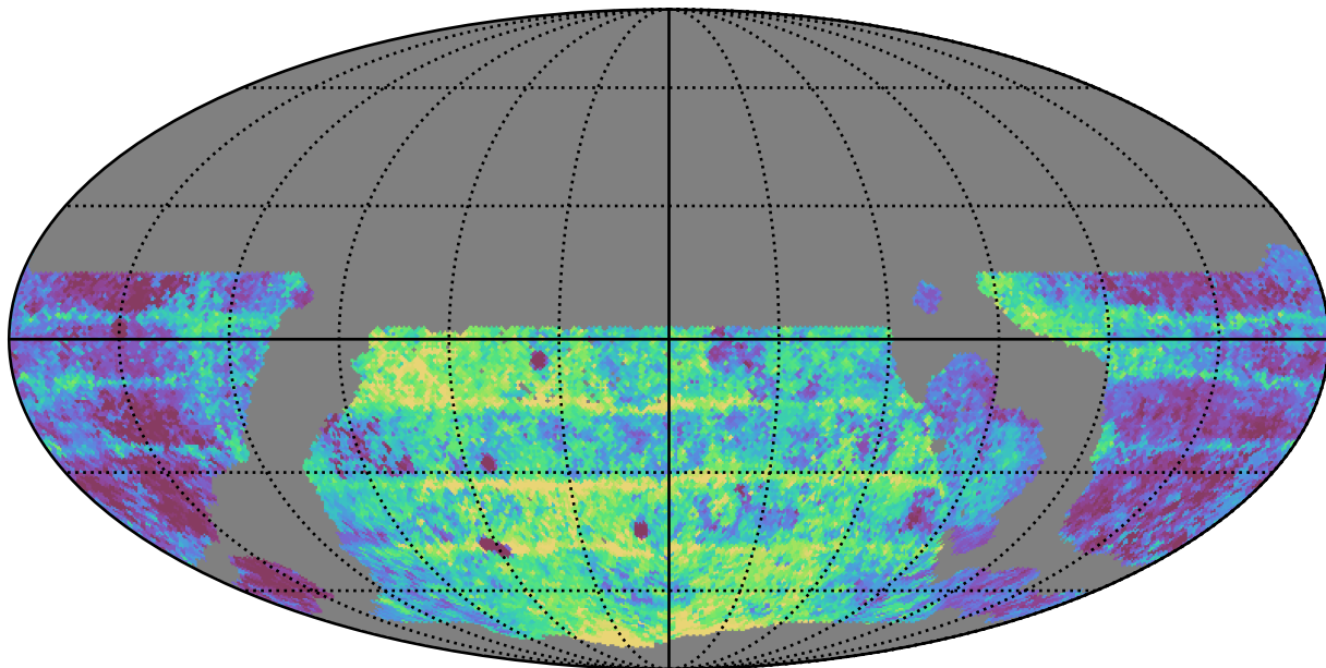
weather_cloudso35v3.4_10yrs WFD g band: Median Inter-Night Gap
