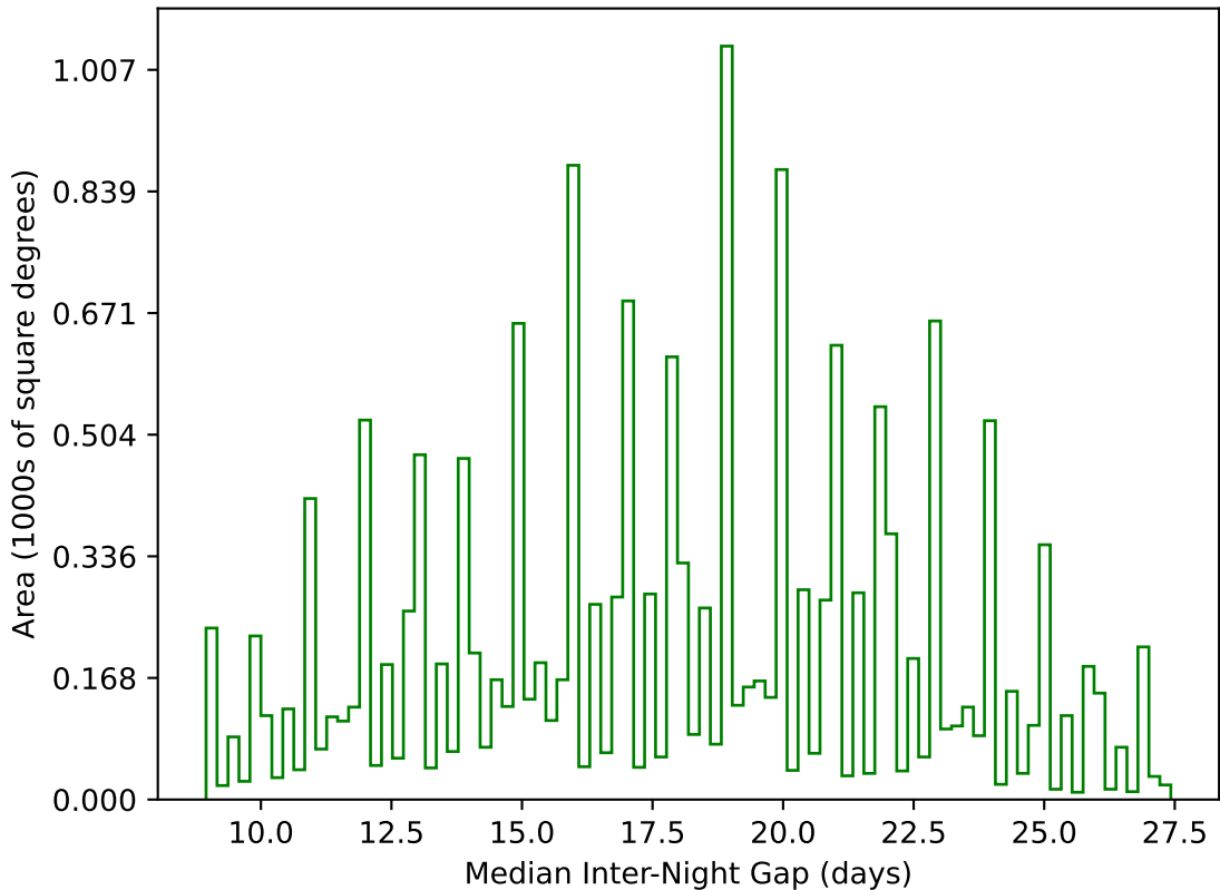
weather_cloudso35v3.4_10yrs WFD g band: Median Inter-Night Gap
