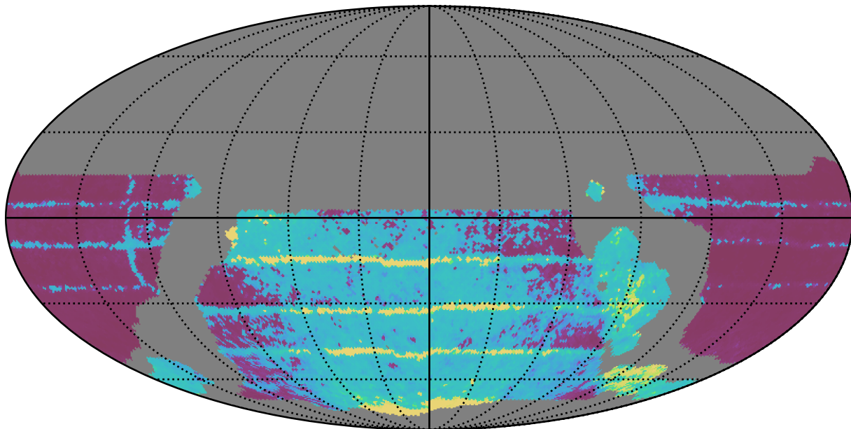
weather_cloudso35v3.4_10yrs WFD all bands: Median Inter-Night Gap
